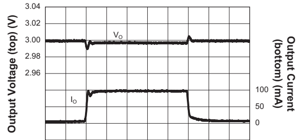
Load Transient Response LDO1
