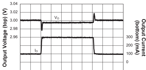
Load Transient Response LDO1
