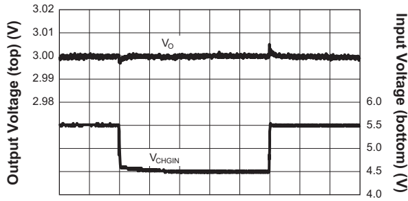
V_{CHGIN} Line Transient Response LDO1
